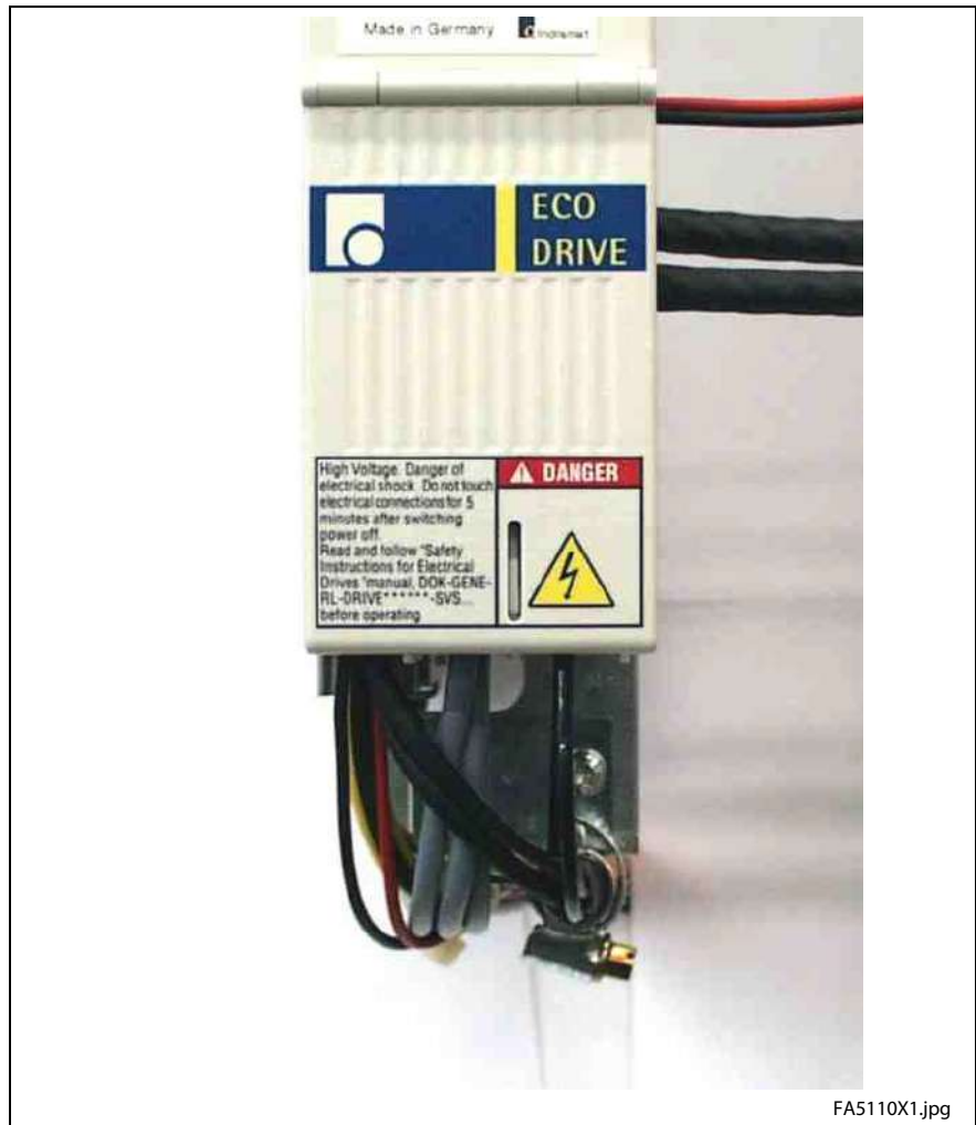
Fig. 16-28: View with contact protection
