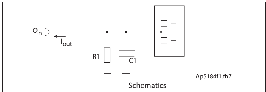
Fig. 5-41: Control outputs
