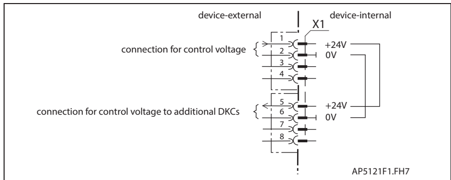
Fig. 6-14: Connections for control voltage
