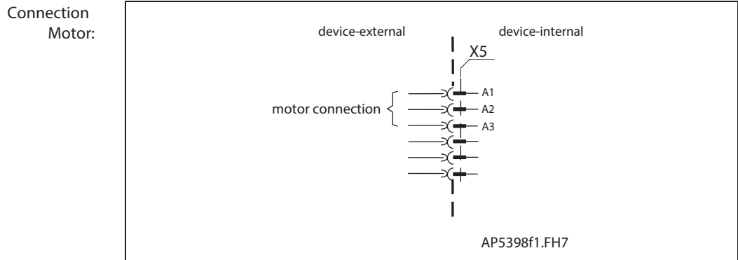
Fig. 5-55: Motor connections
