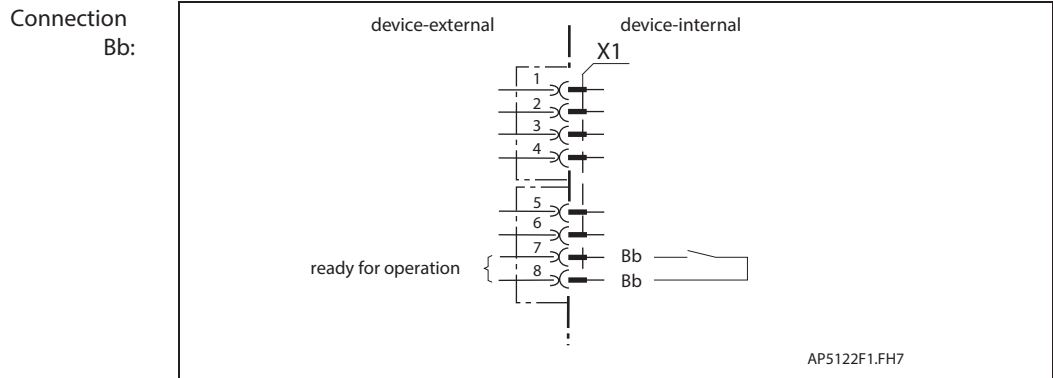
Fig. 4-56: Connections for ready to operate contact
