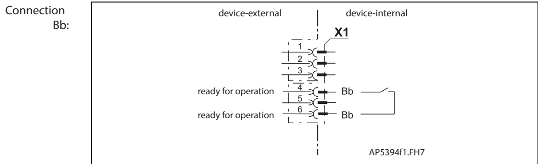
Fig. 5-29: Connections for ready to operate contact
