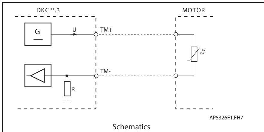
Fig. 4-101: Motor temperature monitoring
