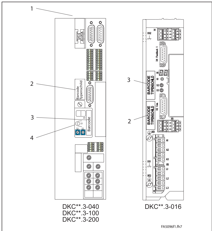
Fig. 14-1: Type plates
