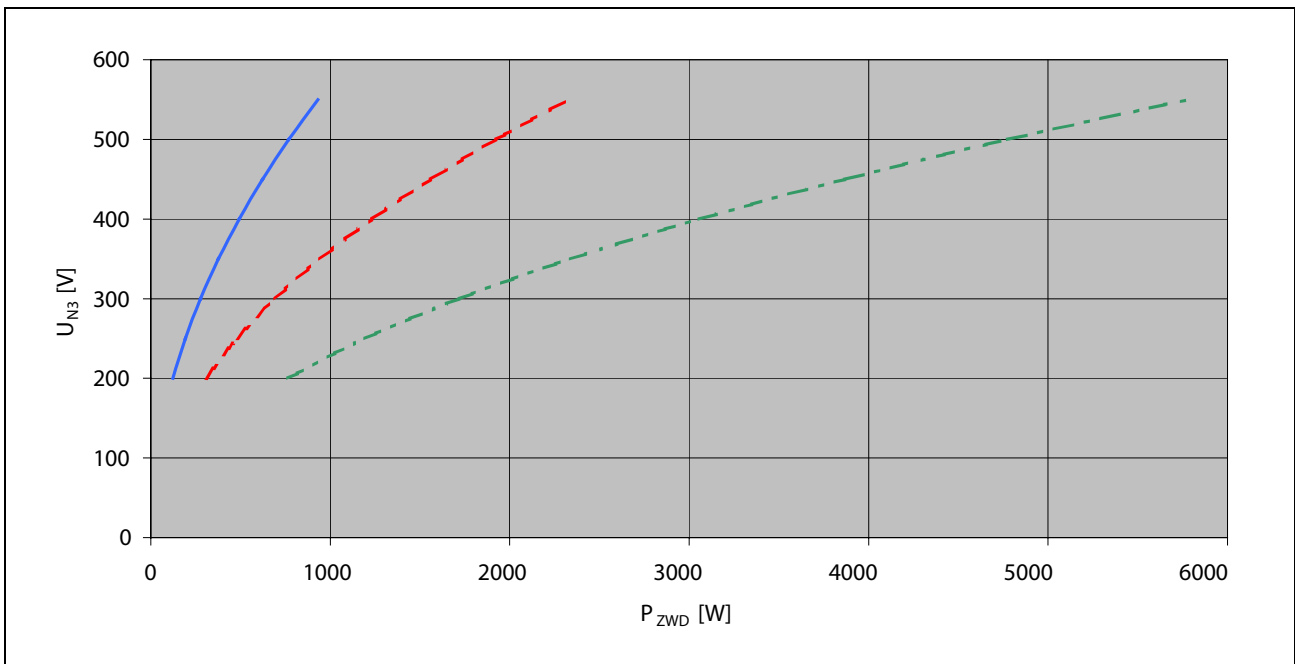
—: DKC**.3-040-7, 60 Hz with / without CZM - - : DKC**.3-100-7, 60 Hz without CZM - - : DKC**.3-100-7, 60 Hz without CZM Fig. 4-38: DC bus continuous power in single-phase mode with 60 Hz
