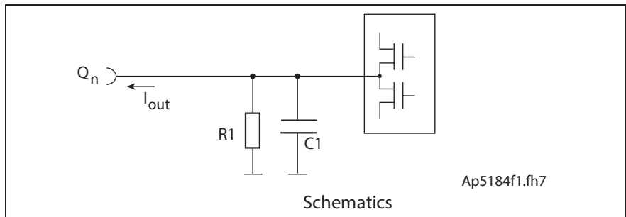
Fig. 6-30: Output circuit
