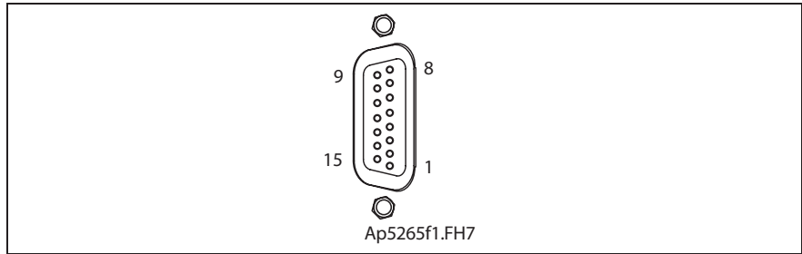
Fig. 4-81: Connector X4
