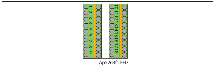
Fig. 4-138: Connector X11
