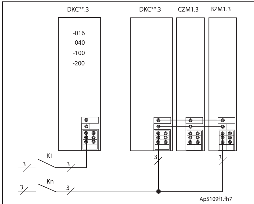
Fig. 4-22: Single source supply
