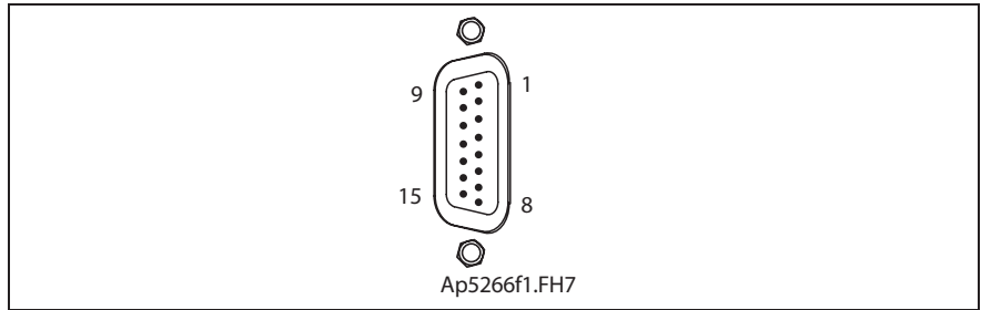
Fig. 4-110: Connector X5
