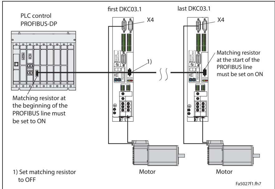
Fig. 4-187: An example of connecting a DKC03.3 to the PLC control via the PROFIBUS-DP
