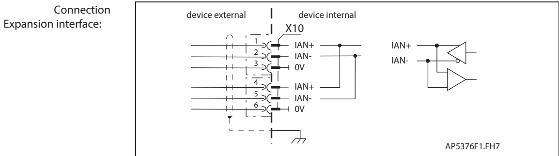
Fig. 4-136: Expansion interface
