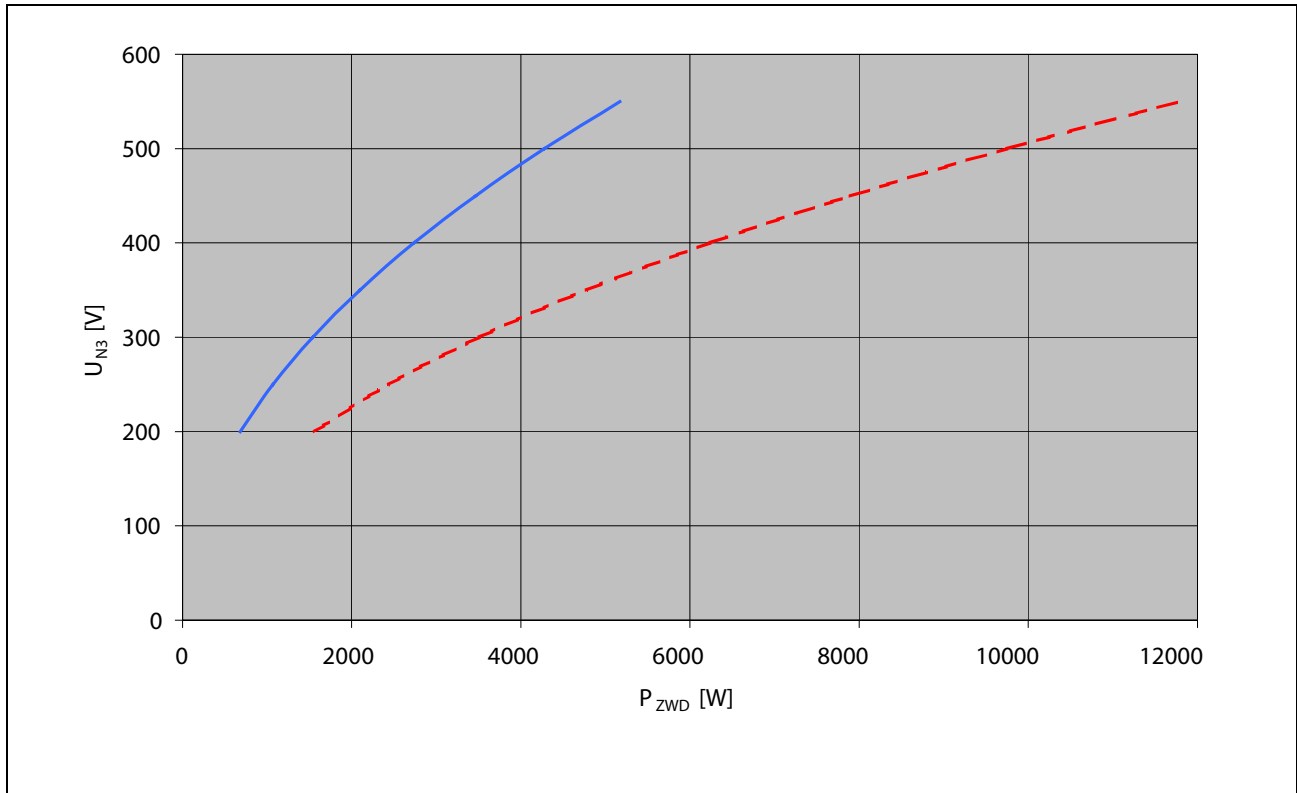
———: DKC**.3-200-7, 60 Hz without CZM - - - - : DKC**.3-200-7, 60 Hz with CZM Fig. 4-39: DC bus continuous power in single-phase mode with 60 Hz
