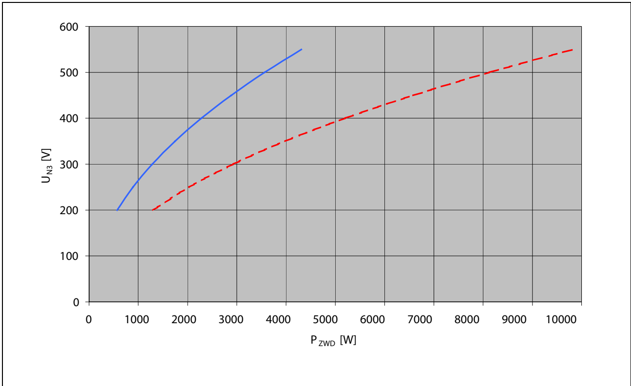
—: DKC**.3-200-7, 50 Hz without CZM - - : DKC**.3-200-7, 50 Hz with CZM Fig. 4-37: Allowed DC bus continuous power in single-phase mode with 50 Hz
